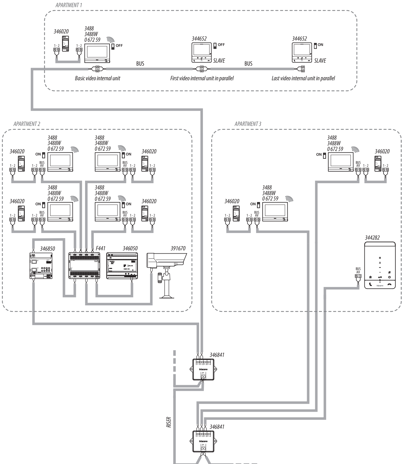
DIAGRAM 3 - EXAMPLE OF MULTI-FAMILY SYSTEM WITH ADDITIONAL INTERNAL UNITS AND POWER SUPPLY
